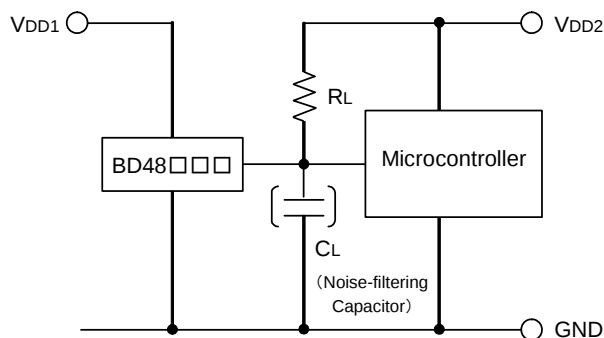
Fig.15 Open Collector Output Type
