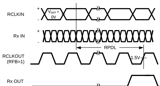
Figure 10. Receiver Propagation Delay
