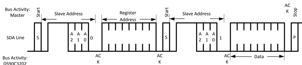
Figure 20. Byte Read
