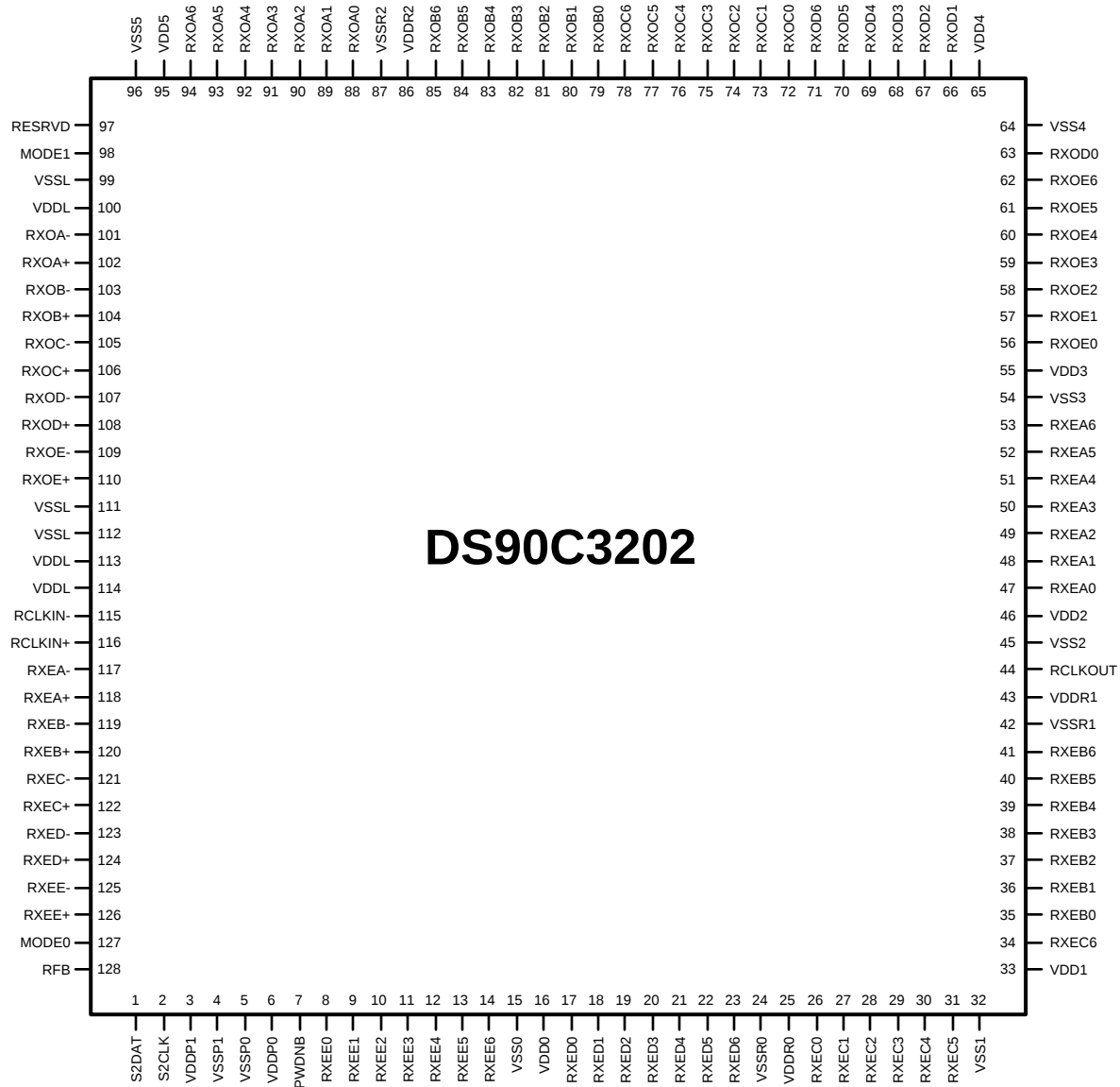
Figure 19. DS90C3202 Receiver
