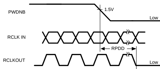
Figure 9. Powerdown Delay
