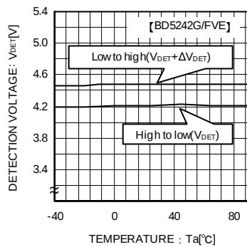
Fig.9 Detection Voltage Release Voltage
