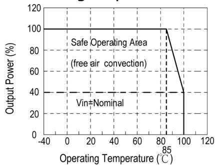
Derating Graph
