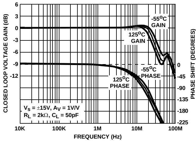
FIGURE 16. FREQUENCY RESPONSE
