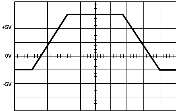
FIGURE 3. LARGE SIGNAL TRANSIENT RESPONSE
