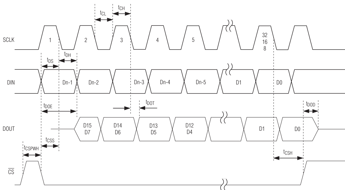
Figure 10. DAC/GPIO Serial-Interface Timing (Clock Modes 00, 01, and 10)
