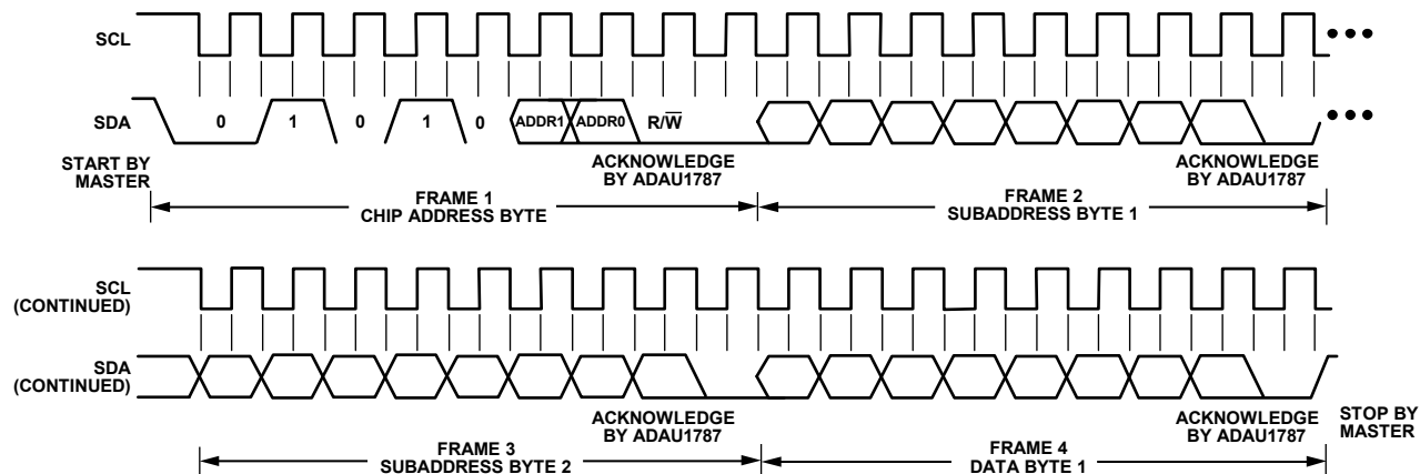
Figure 59. I 2 C Write to ADAU1787 Clocking
