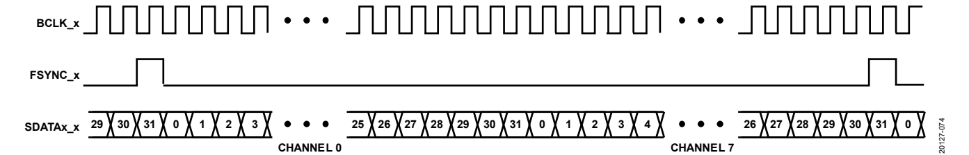
Figure 69. 8-Channel TDM Mode, Default Settings, Except SPTx_SAI_MODE = 1
