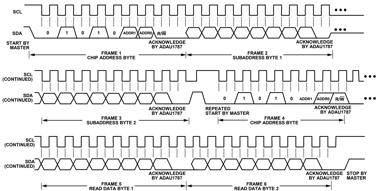
Figure 60. I 2 C Read from ADAU1787 Clocking
