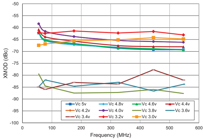
XMOD versus Frequency, 79 Channel 39dBmV Flat Input, Temp=+25°C
