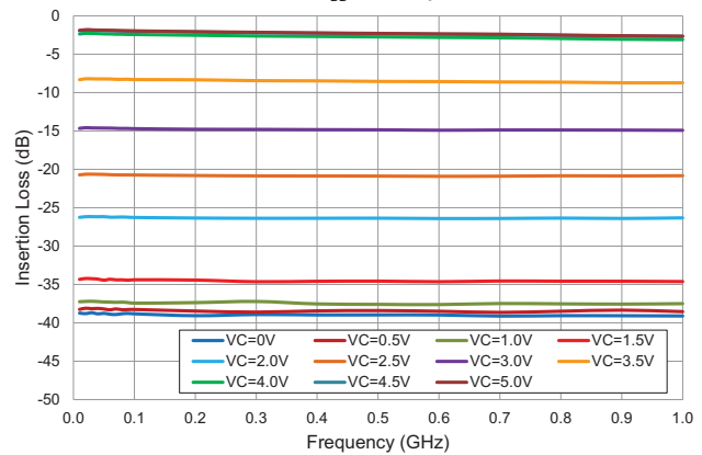
Insertion Loss versus Frequency RFSA3013, V_{DD}=5V , Temp=+25°C
