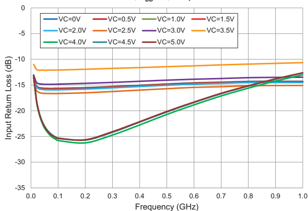
Input Return Loss versus Frequency RFSA3013, V_{DD}=5V , Temp=+25°C
