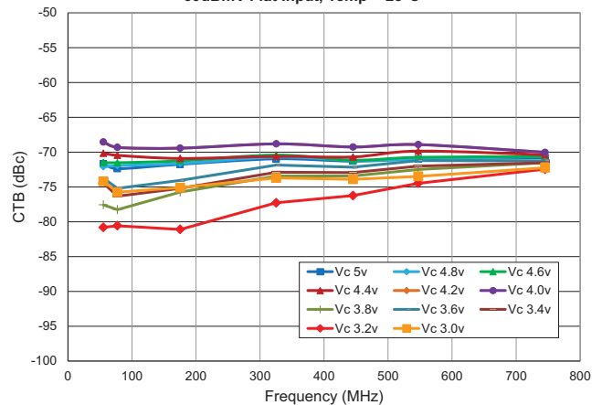
CTB versus Frequency, 112 Channel 39dBmV Flat Input, Temp=+25°C
