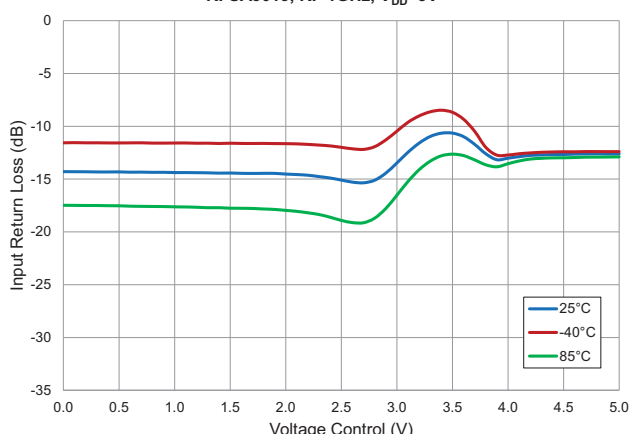
Input Return Loss versus Voltage Control RFSA3013, RF 1GHz, V_{DD}=5V
