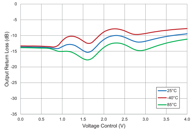
Output Return Loss versus Voltage Control RFSA3013, RF 1GHz, V_{DD}=5V
