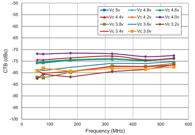
CTB versus Frequency, 79 Channel 39dBmV Flat Input, Temp=+25°C
