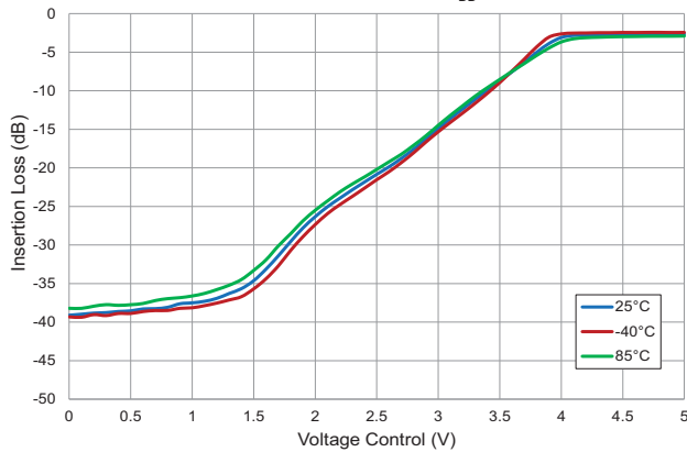
Insertion Loss versus Voltage Control RFSA3013, RF 1GHz, V_{DD}=5V
