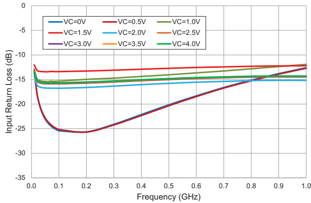
Input Return Loss versus Frequency RFSA3013, V_{DD}=5V , Temp=+25°C
