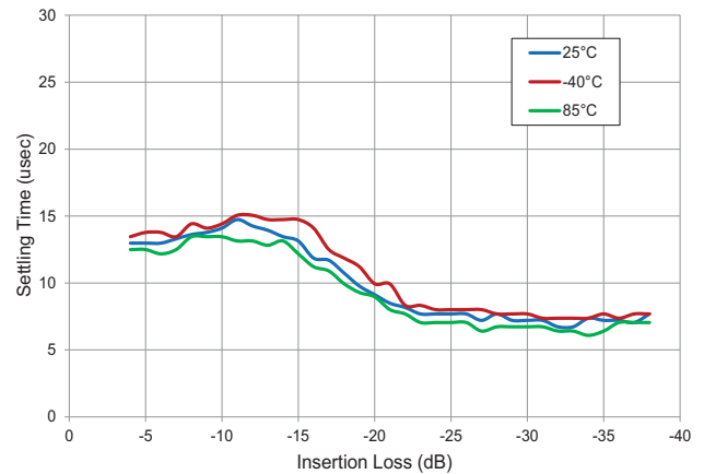
Settling Time versus Insertion Loss 1dB Steps, RF 1GHz, V_{DD}=5V
