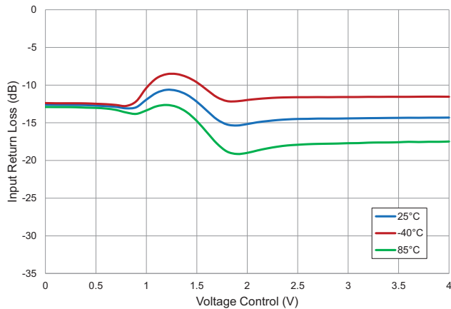
Input Return Loss versus Voltage Control RFSA3013, RF 1GHz, V_{DD}=5V
