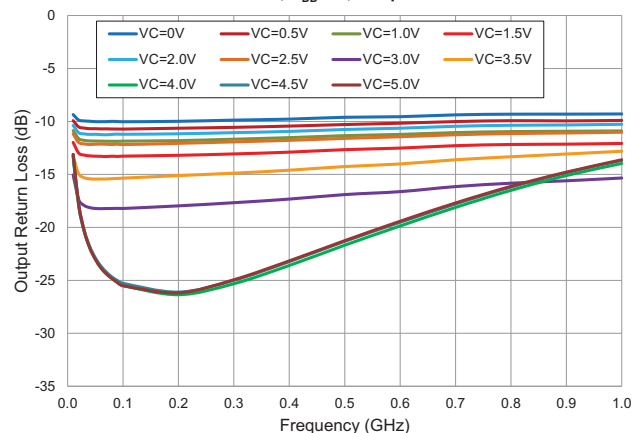
Output Return Loss versus Frequency RFSA3013, V_{DD}=5V , Temp=+25°C
