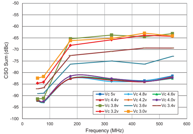
CSO Sum versus Frequency, 79 Channel 39dBmV Flat Input, Temp=+25°C
