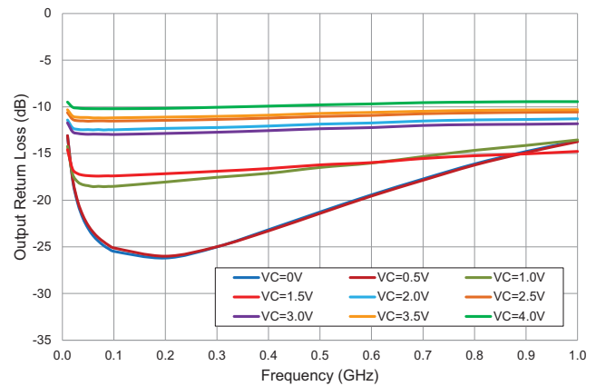
Output Return Loss versus Frequency RFSA3013, V_{DD}=5V , Temp=+25°C
