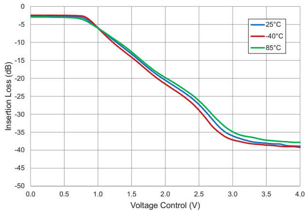
Insertion Loss versus Voltage Control RFSA3013, RF 1GHz, V_{DD}=5V
