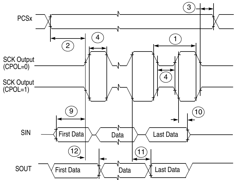
Figure 34. DSPI classic SPI timing — slave, CPHA = 1
