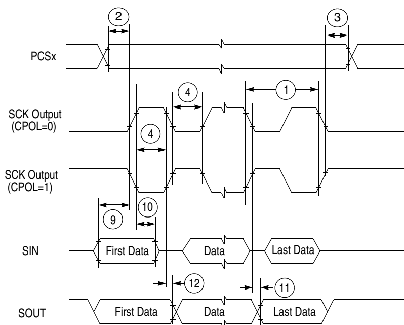
Figure 31. DSPI classic SPI timing — master, CPHA = 0
