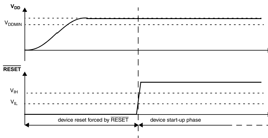
Figure 21. Start-up reset requirements
