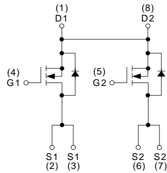
N-Channel MOSFET
