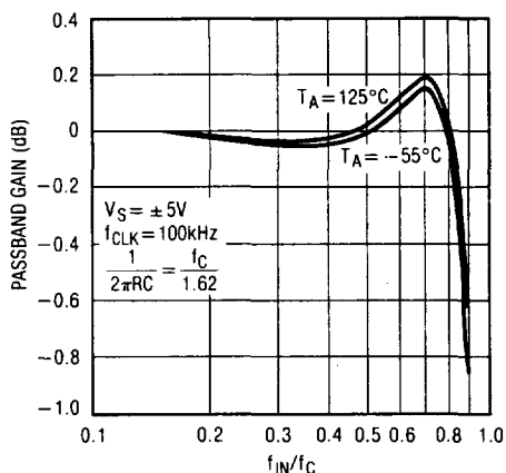
Passband Gain vs Input Frequency
