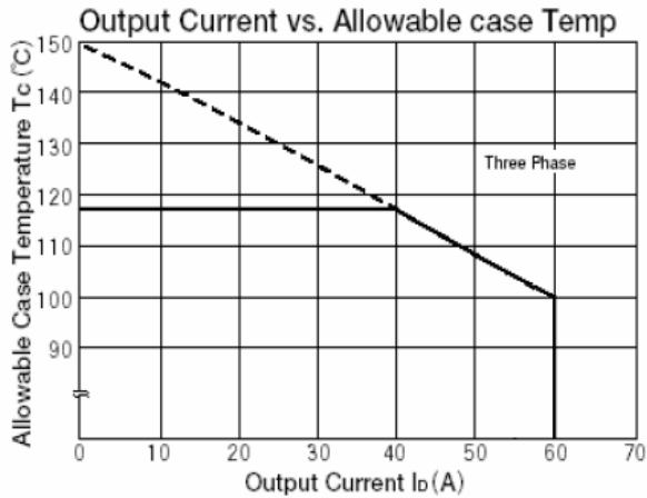
Fig.1. Output Current vs. Allowable case Temp
