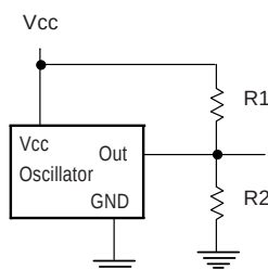
Thevenin Equivalent Termination
