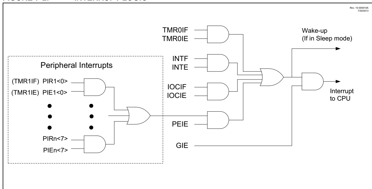
FIGURE 7-1: INTERRUPT LOGIC
