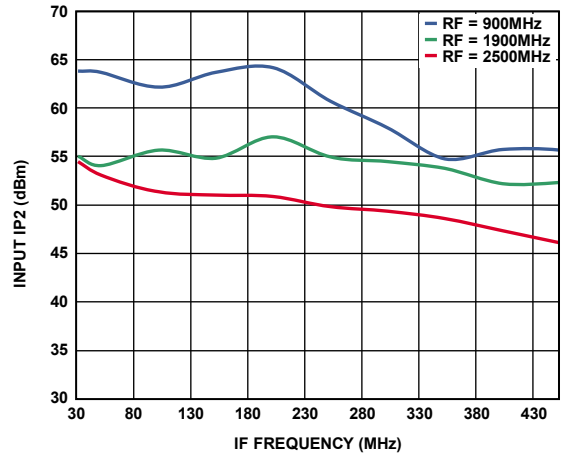
Figure 19. Input IP2 vs. IF Frequency
