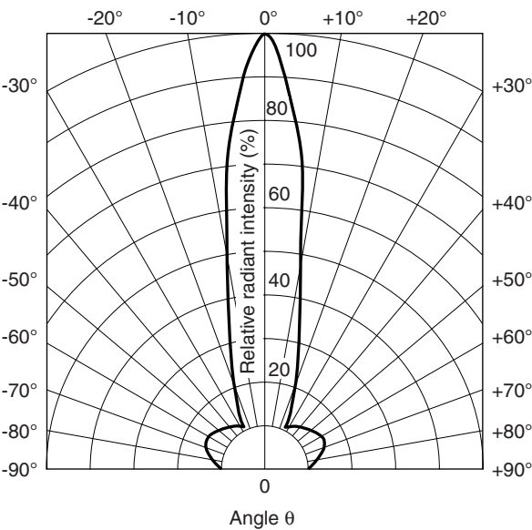
Fig. 2 Radiation Diagram
