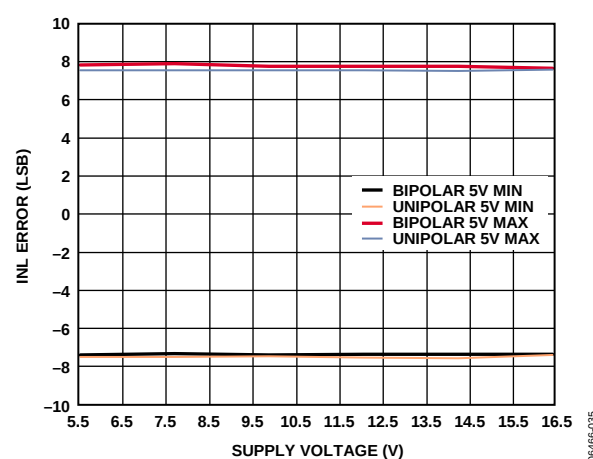
Figure 16. AD5752R Integral Nonlinearity Error vs. Supply Voltage
