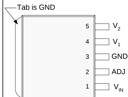
DF PACKAGE (Top View)
