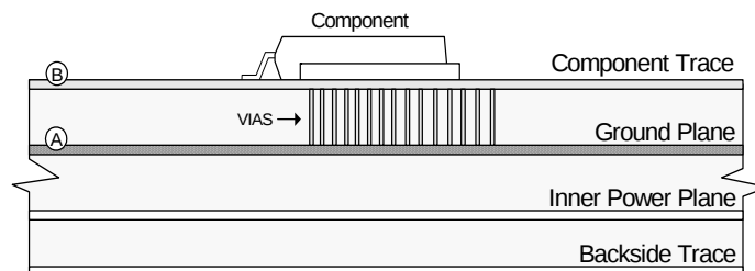
Figure 3 - Heatsink
