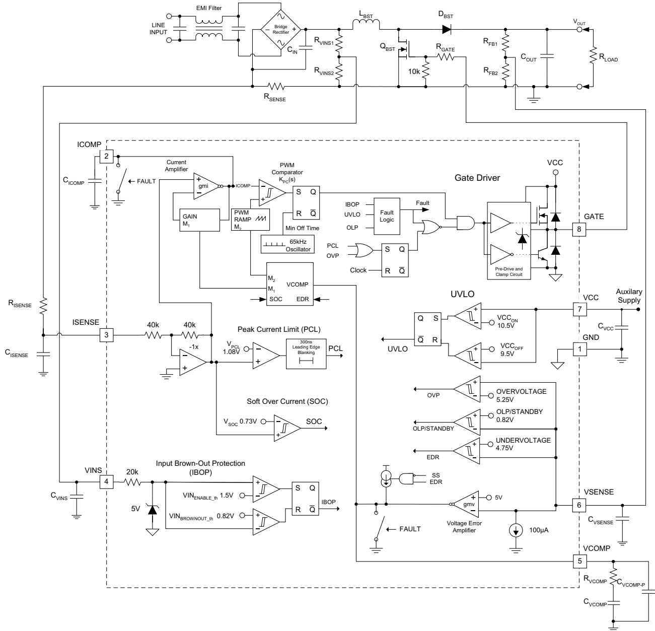
Figure 18. Block Diagram
