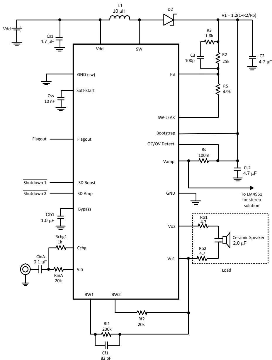
Figure 3. Typical Audio Amplifier Application Circuit
