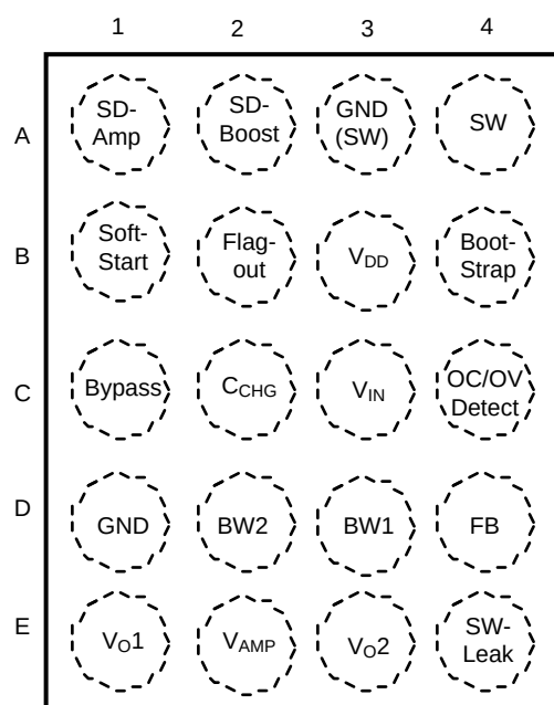
Figure 1. micro SMD Package (Top View)
