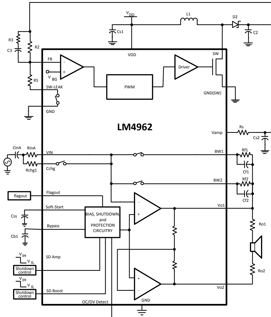
Figure 4. LM4962 Block Diagram
