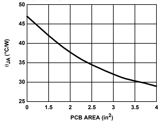
FIGURE 8. EL7563CRE THERMAL RESISTANCE vs PCB AREA - NO AIR FLOW
