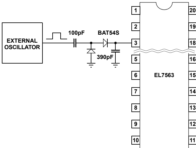
FIGURE 22. OSCILLATOR SYNCHRONIZATION
