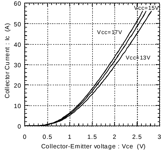
Collector current vs. Collector-Emmitter voltage Tj=125°C
