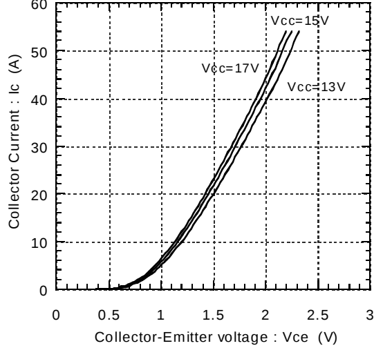
Collector current vs. Collector-Emmitter voltage Tj=25°C
