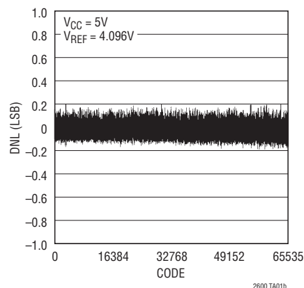
Differential Nonlinearity (LTC2601)
