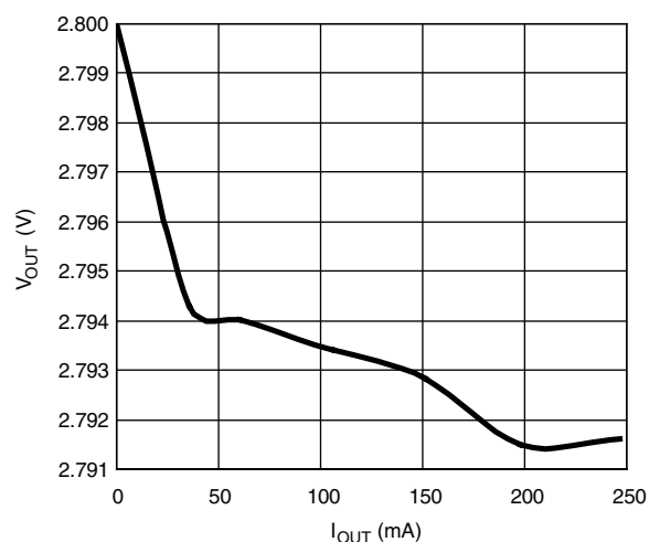
Load Regulation
