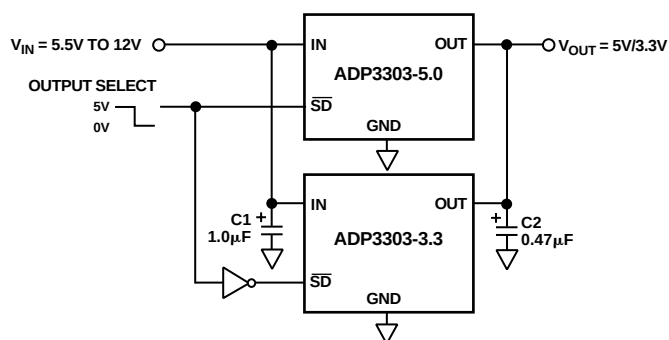
Figure 23. Crossover Switch
