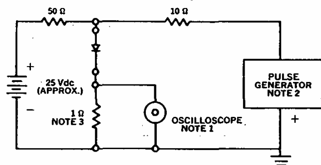
Reverse-Recovery Circuit
