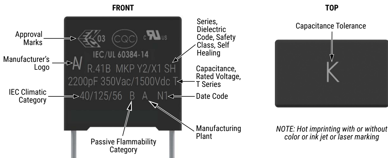
Manufacturing Date Code (IEC 60062)
