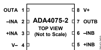
Figure 2. 8-Lead, 2 mm × 2 mm LFCSP
