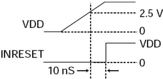
Figure 3: Reset Timing
