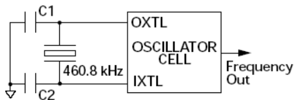
Figure 9: Crystal Oscillator
