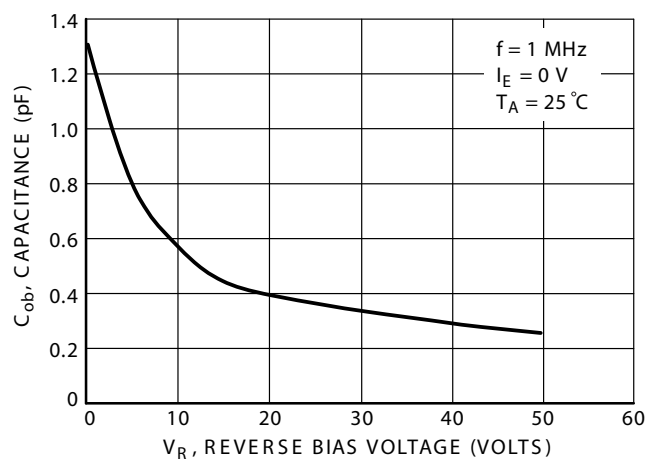
FIG. 69 Output Capacitance
