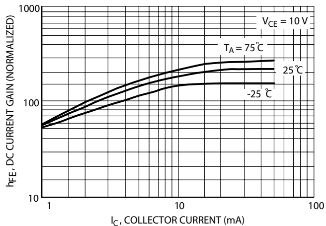
FIG.13 DC Current Gain
