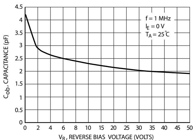
FIG.19 Output Capacitance
