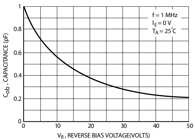
FIG.14 Output Capacitance
