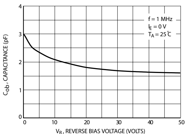
FIG.9 Output Capacitance
