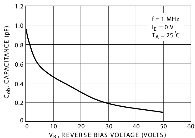
FIG.64 Output Capacitance
