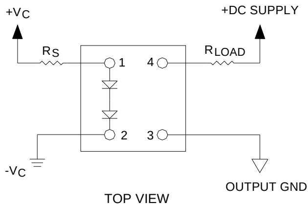
Figure 2. Terminal Connections
