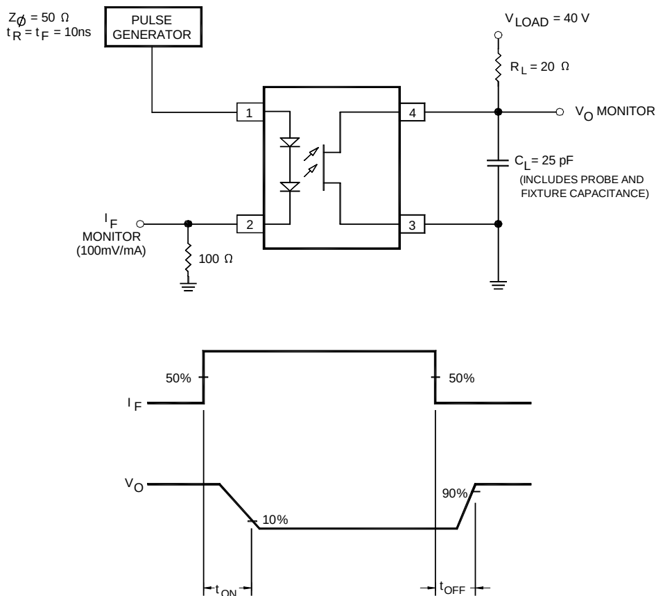
Figure 3. Switching Waveforms and Test Circuits
