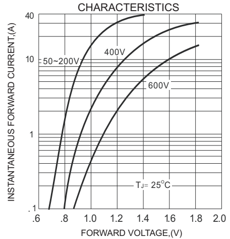
FIG.3-TYPICAL FORWARD
