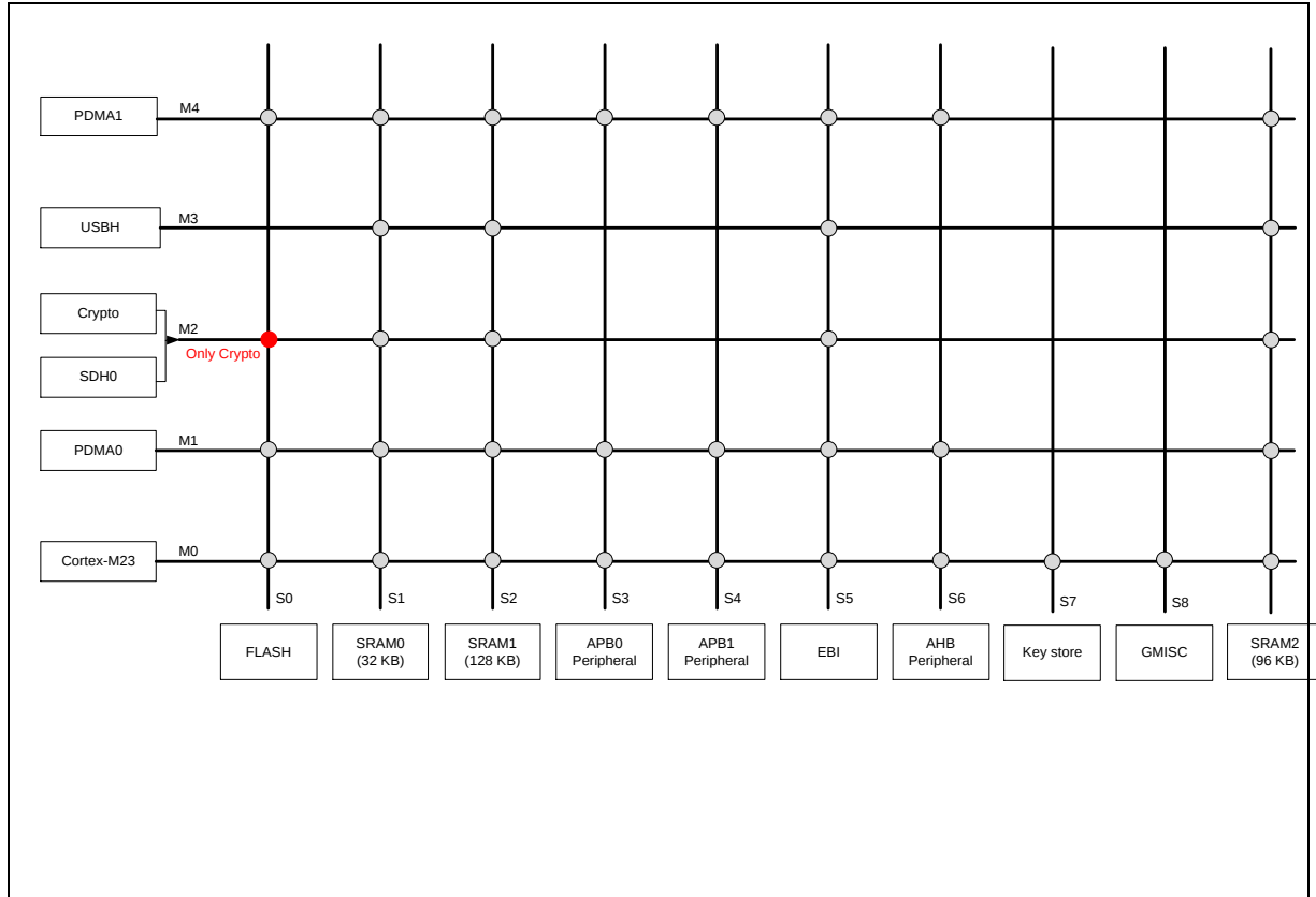
Figure 6.2-2 M2354 Bus Matrix Architecture Diagram
