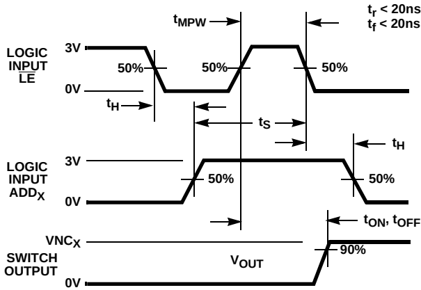
FIGURE 3. BREAK-BEFORE-MAKE TIME
