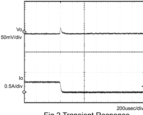
Fig.2 Transient Response (0.5→0A) Co=1µF
