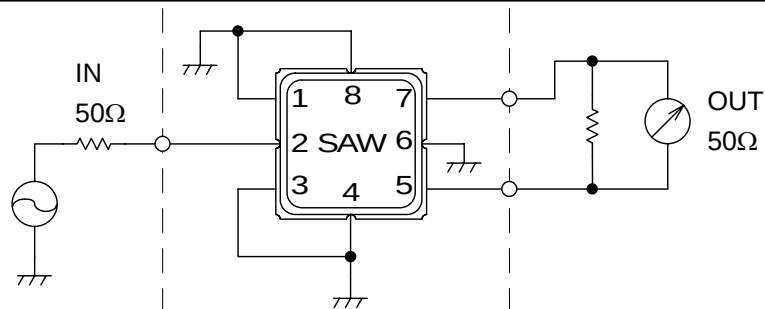
Fig.1 Measuring circuit
