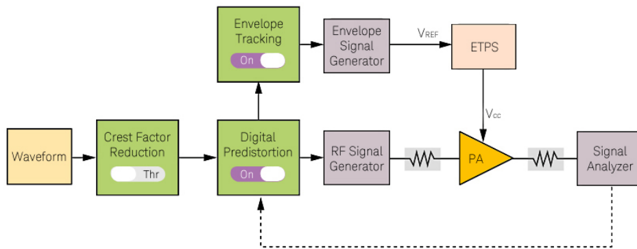
Figure 17. ET can be chosen from a non-predistorted waveform or pre-distorted waveform
