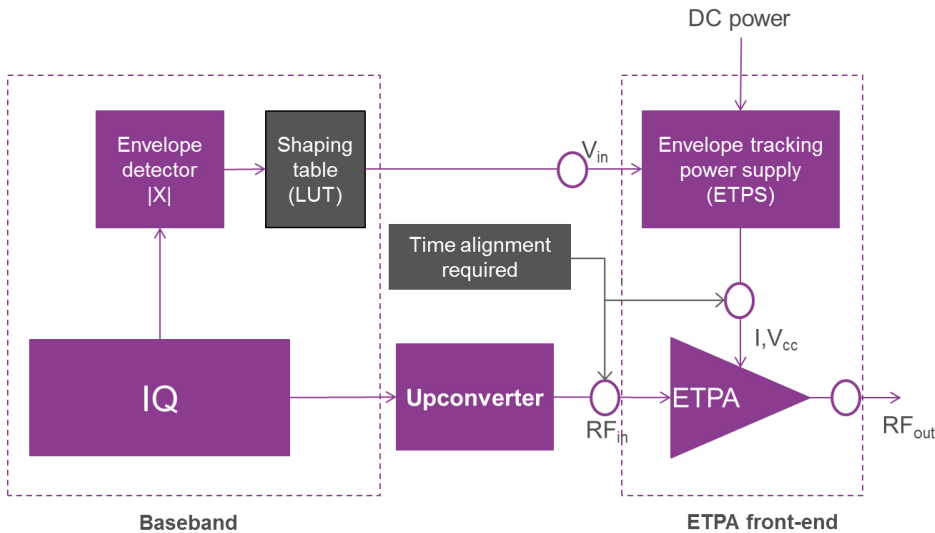
Figure 12. Envelope tracking system simplified block diagram
