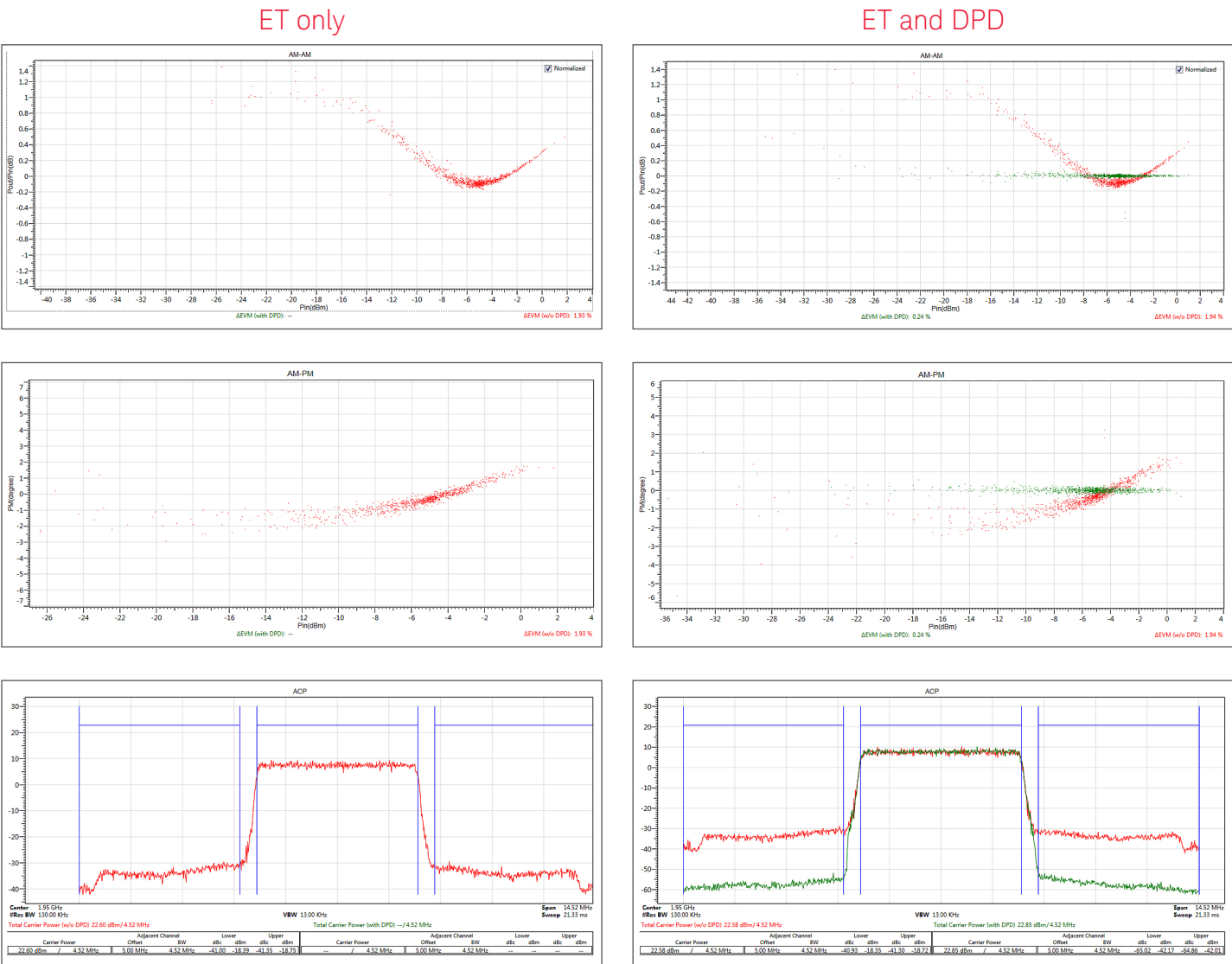
Figure 18. These graphs show the effect of ET only and ET with DPD with AM-AM, AM-PM and ACP results
