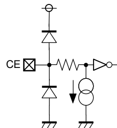
CE Pin Equivalent Circuit Diagram
