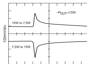
50 \mu s/div 25% \leftrightarrow 50% SMTR2815D +VOUT STEP LOAD RESPONSE
