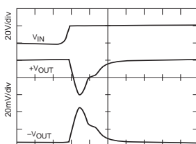
50 \mu s/div 16 TO 40V SMTR2815D STEP LINE RESPONSE
