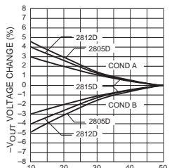
COND. B: 50% LOAD +V, 50% TO 10% -V COND. A: 50% LOAD -V, 50% TO 10% +V CROSS REGULATION
