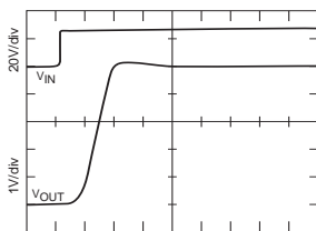
500 \mu s/div SMTR2805S TURN-ON INTO NO LOAD
