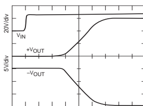
200 \mu s/div SMTR2815D TURN-ON INTO NO LOAD
