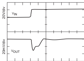
50 \mu s/div 16 TO 40V SMTR2805S STEP LINE RESPONSE
