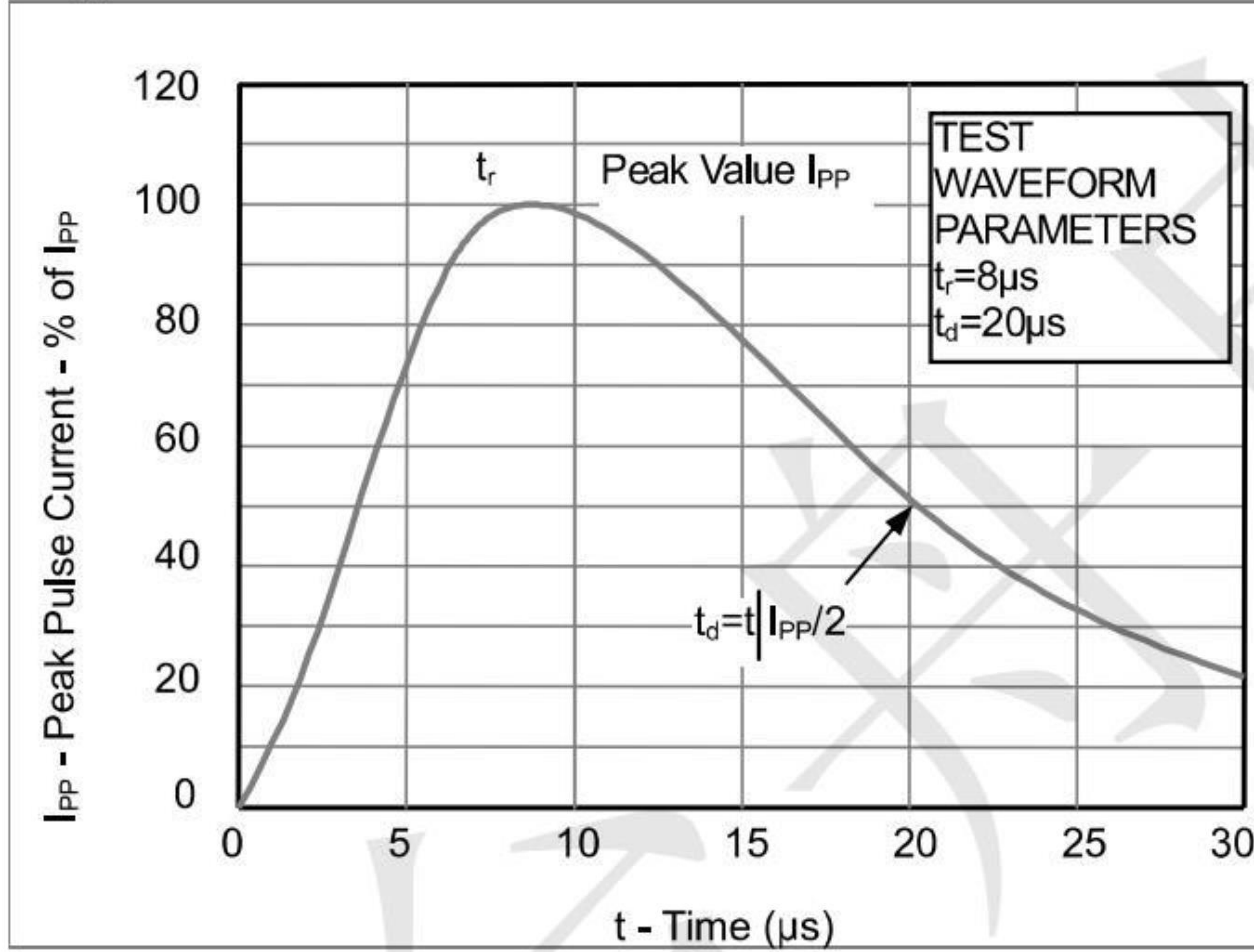
Fig1. 8/20 \mu\text{s} Pulse Waveform
