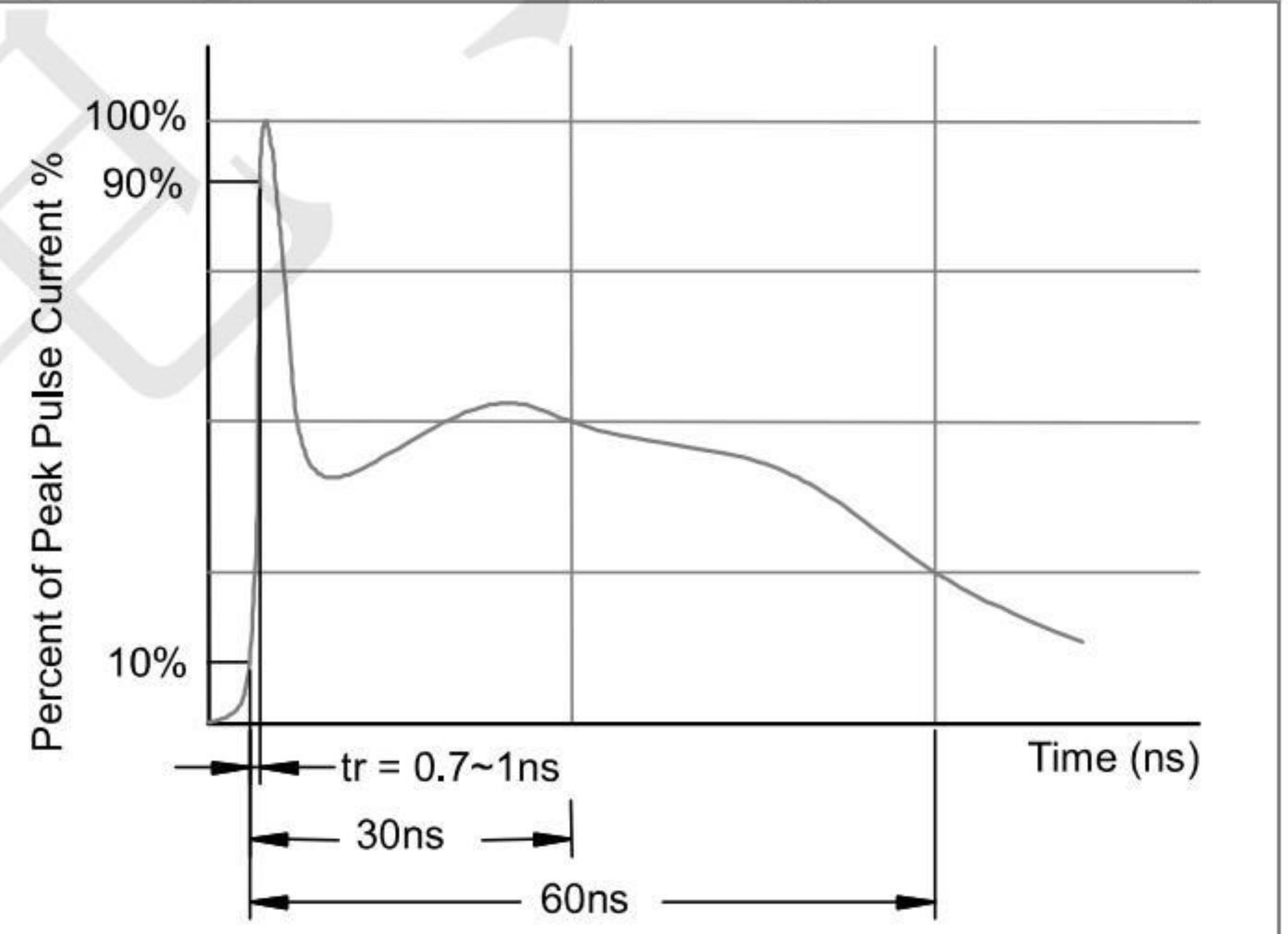
Fig2. ESD Pulse Waveform (according to IEC 61000-4-2)
