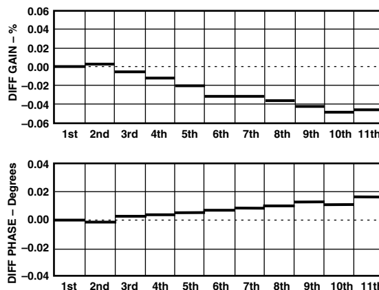
TPC 22. AD8036 Differential Gain and Phase Error, G = +1 , R_L = 150\Omega , F = 3.58 MHz
