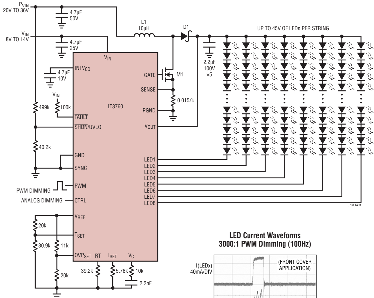
92% Efficient, 36W LED Driver, 1MHz Boost, 8 Strings, 100mA Per String
