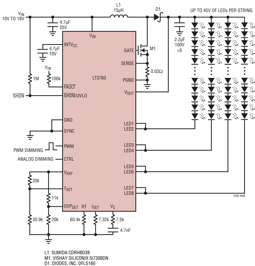
29W LED Driver, 700kHz Boost, 4 Strings, 160mA Per String
