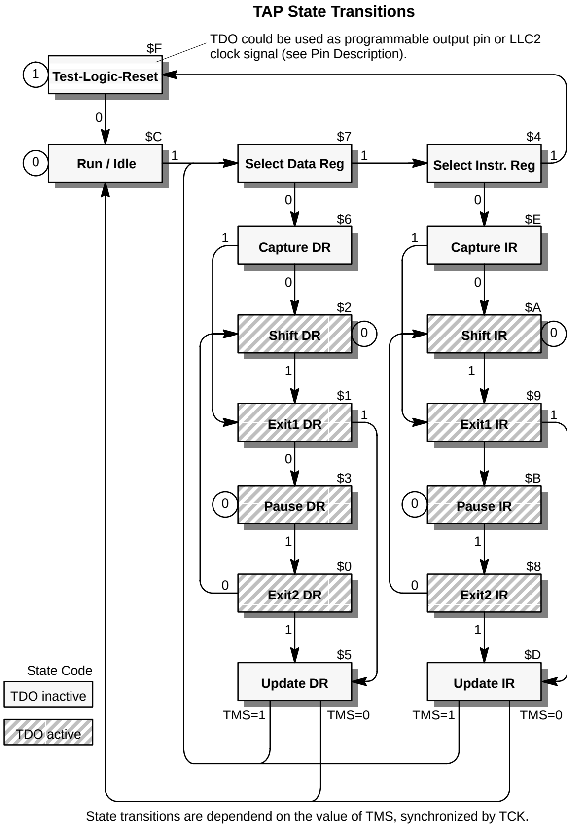
Fig. 2-43: TAP state transitions
