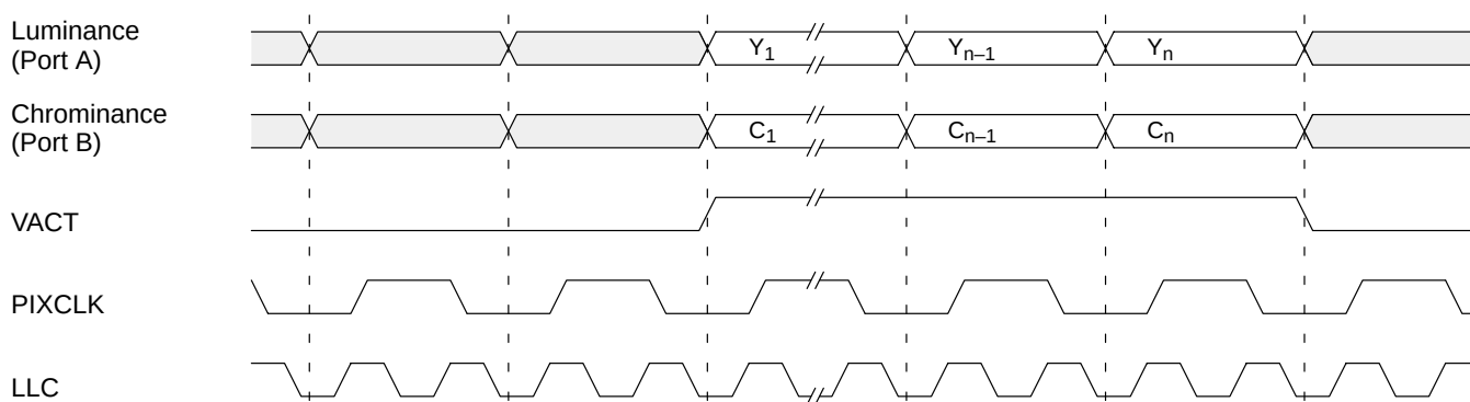
Fig. 2–24: Output timing in single clock mode
