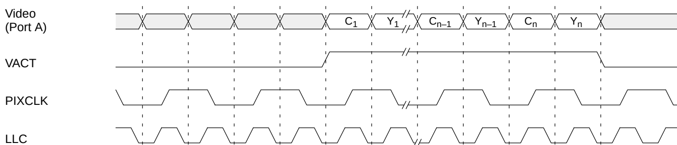
Fig. 2–25: Output timing in double clock mode
