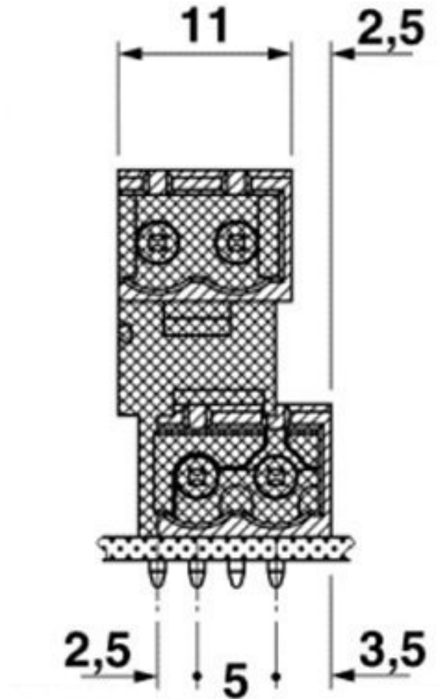
Dimensioned drawing
