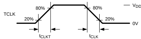
Figure 4. Serializer Input Clock Transition Times
