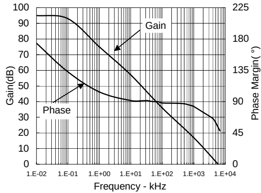
Open Loop Gain & Phase Margin vs. Frequency
