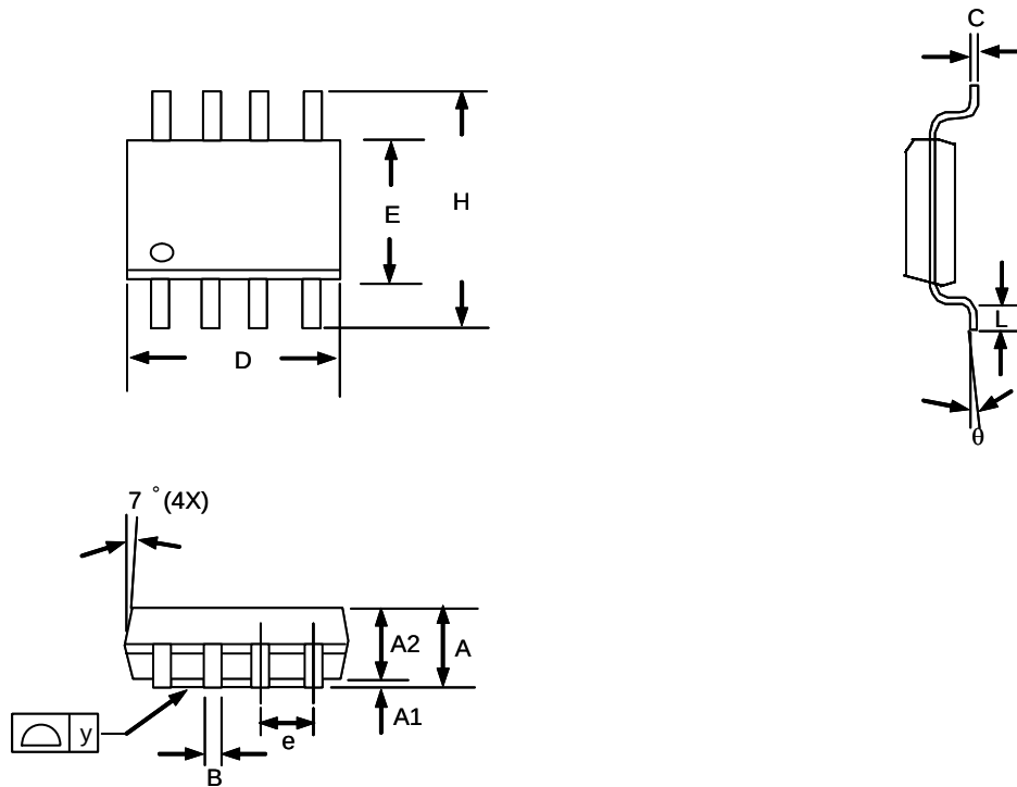
SOP- 8 (P1) Package
