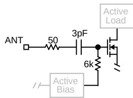
Figure 1. ANT Pin
