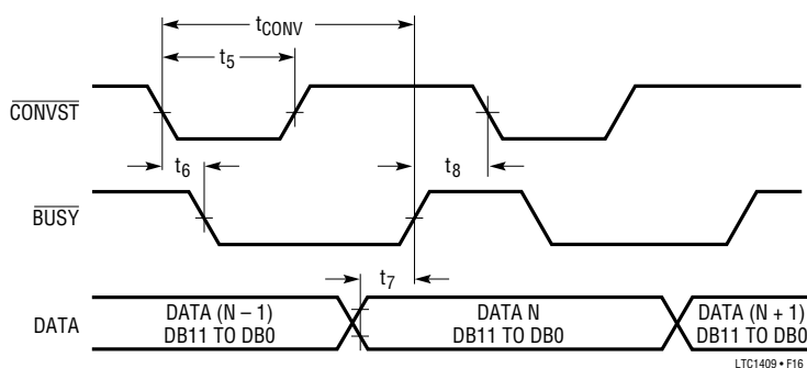
Figure 16. Mode 1a. \overline{\text{CONVST}} Starts a Conversion. Data Outputs Always Enabled ( \overline{\text{CONVST}} = \text{low} )
