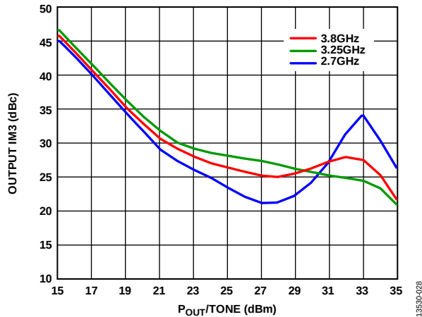
Figure 26. Output Third-Order Intermodulation (IM3) vs. P_{OUT}/Tone at V_{DD} = 25\text{ V}
