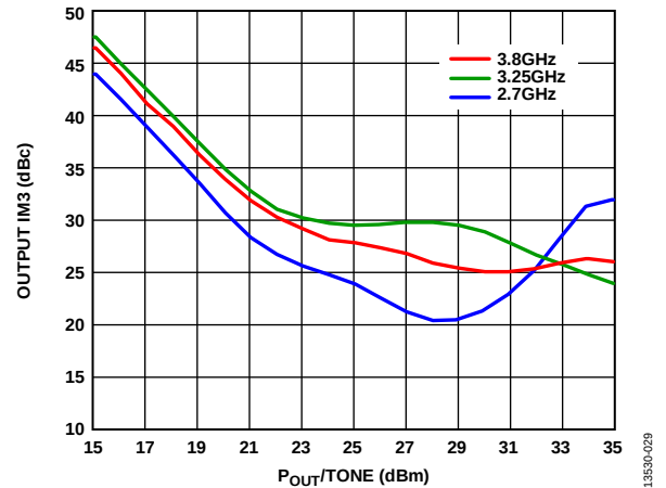
Figure 29. Output Third-Order Intermodulation (IM3) vs. P_{OUT}/Tone at V_{DD} = 32\text{ V}
