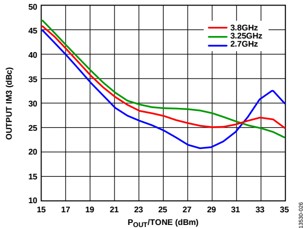
Figure 27. Output Third-Order Intermodulation (IM3) vs. P_{OUT}/Tone at V_{DD} = 28\text{ V}
