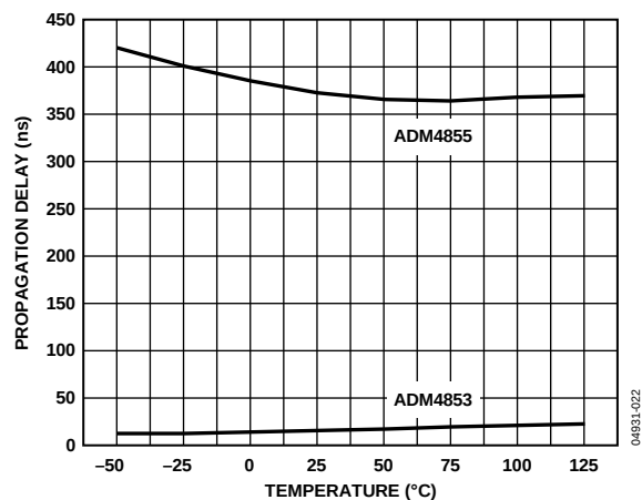
Figure 15. Driver Propagation Delay vs. Temperature (ADM4853/ADM4855)
