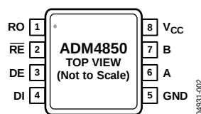
Figure 3. ADM4850, 8-Lead MSOP, Pin Configuration
