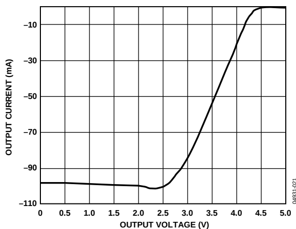
Figure 14. Output Current vs. Driver Output High Voltage
